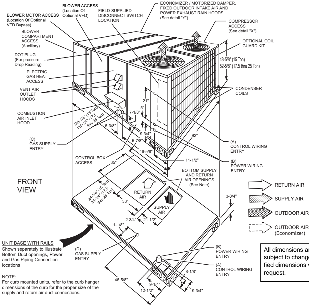
FIGURE 4 - UNIT DIMENSIONS DH180, 210, 240 & 300 (FRONT VIEW)
