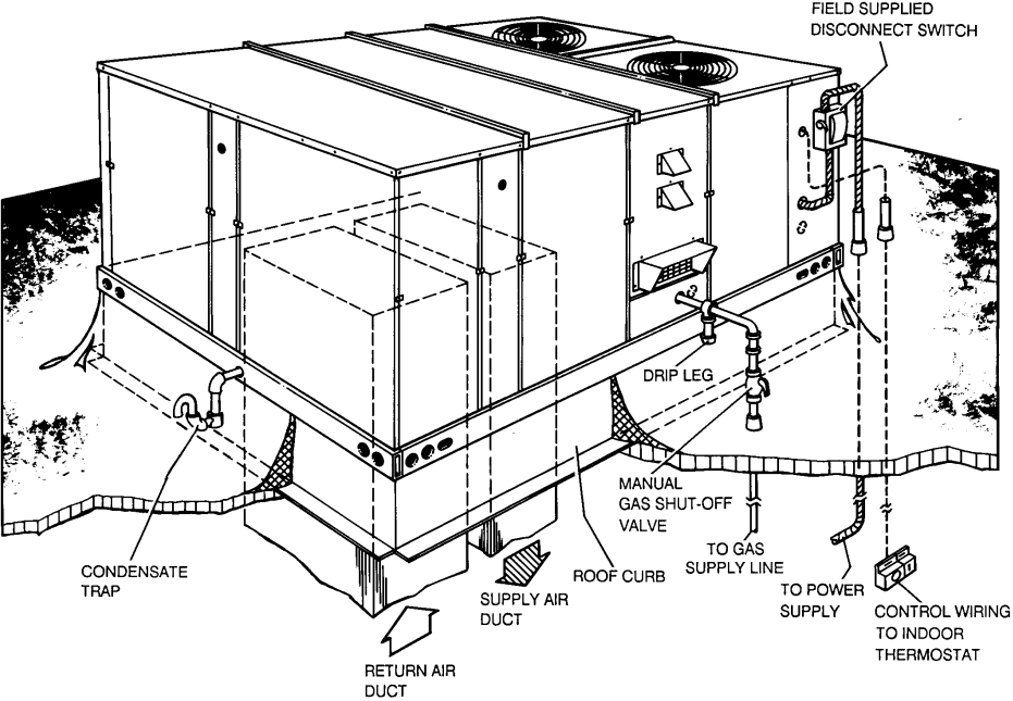
FIGURE 14 - TYPICAL ROOFTOP INSTALLATION
