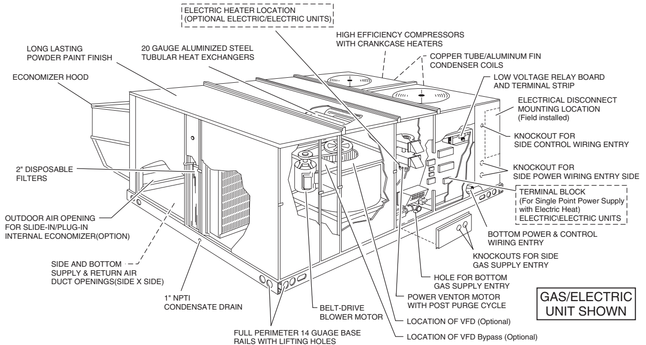
FIGURE 1 - UNIT CUTAWAY
