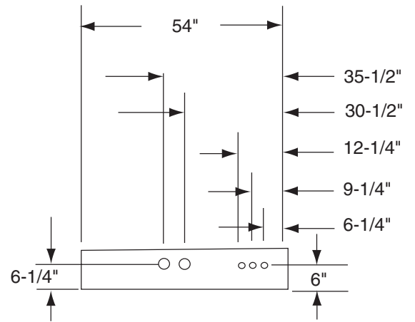
PANEL B 3/4" K.O. (CONTROL WIRING)
