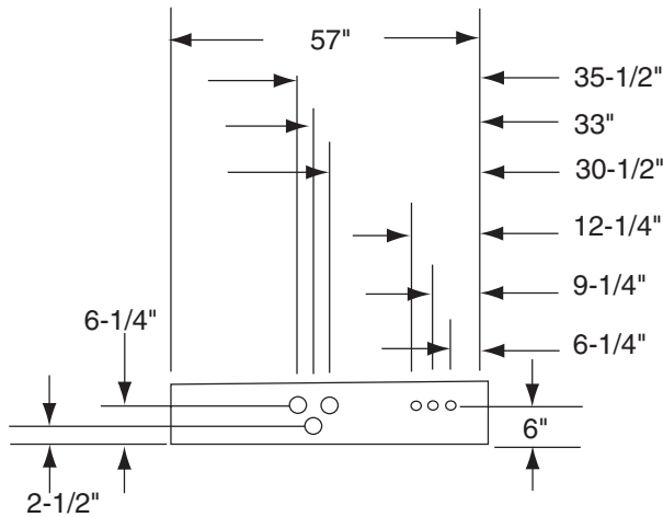
PANEL A 3/4" K.O. (CONTROL WIRING)
