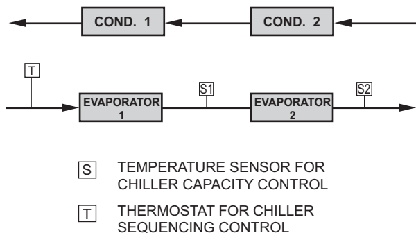
FIG. 3 – SERIES COUNTERFLOW
