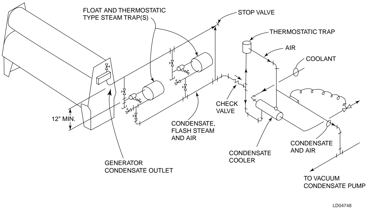
FIG. 7 – SYSTEM 3: VACUUM CONDENSATE RETURN SYSTEM.
