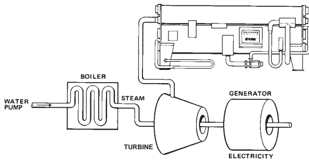
COGENERATION
