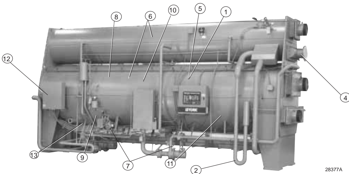
FIG. 1 – MILLENNIUM SINGLE-STAGE ABSORPTION CHILLER RELIABILITY FEATURES
