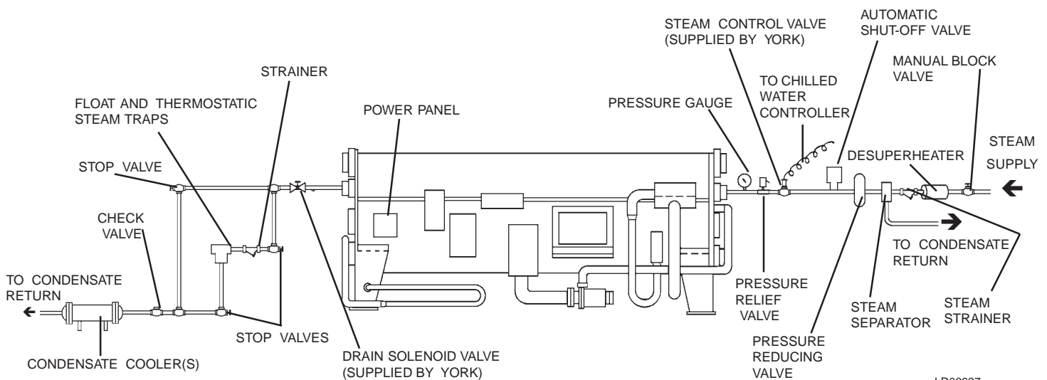
FIG. 4 – TYPICAL STEAM PIPING 20
