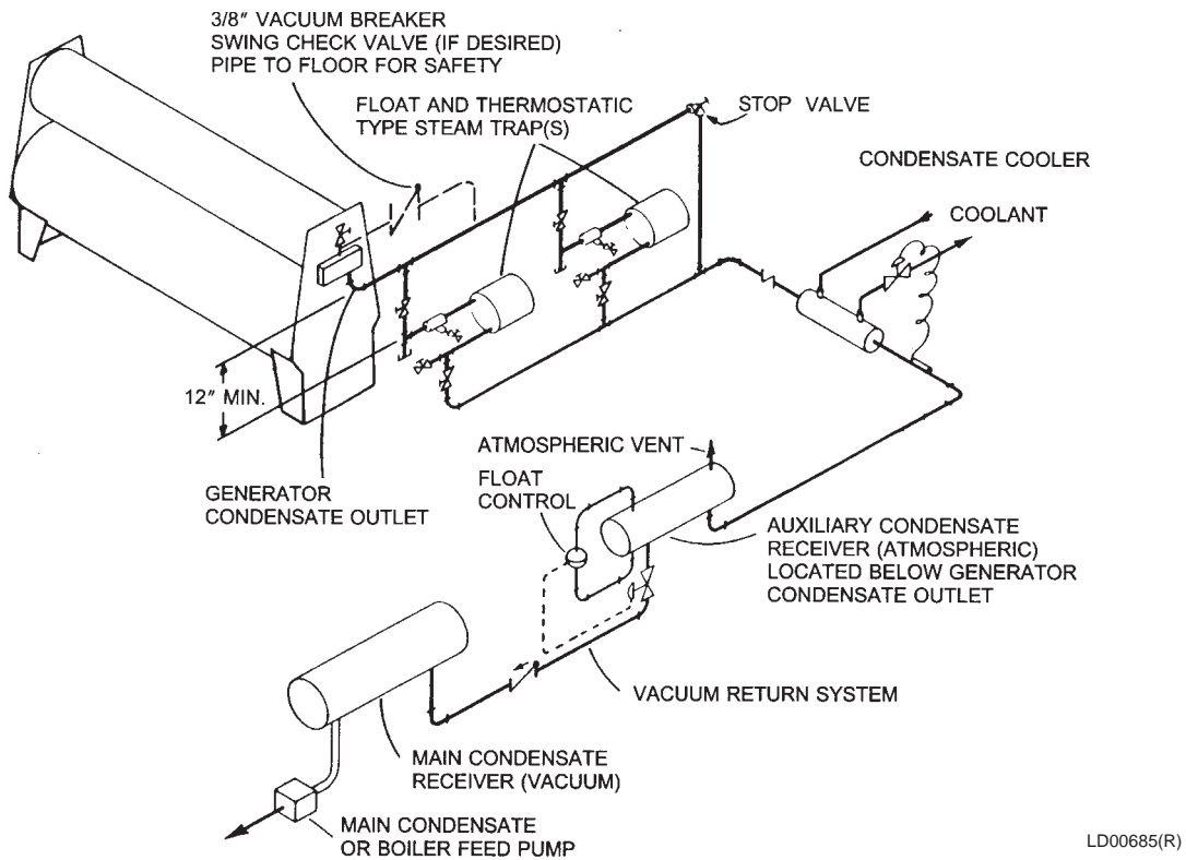
FIG. 6 – SYSTEM 2: VACUUM CONDENSATE RETURN SYSTEM
