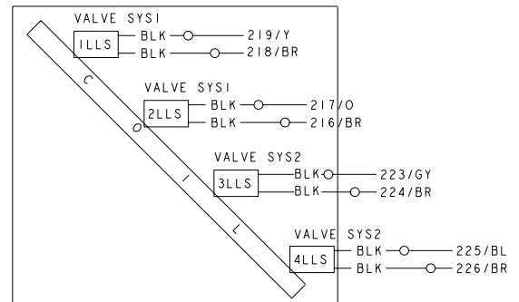
FIGURE 7 - 30, 40 & 50 TON LIQUID LINE SOLENOID WIRING
